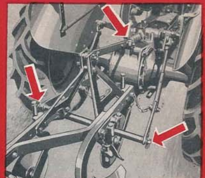
New Hydraulic Touch Control and linkage combined with added attachment lugs and provisioned for attaching a swinging draw bar permit use of more equipment with greater safety.
