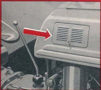
New screened air intake grille easily removed for cleaning by loosening a single wing nut. Extension stack easily attached when desired as optional equipment.
