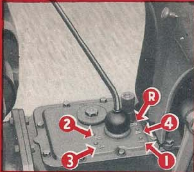
New 4-speed transmission provides higher speed, with choice of speeds. Quiet operation, smooth easy shifting. Inspection plate easily removable.
